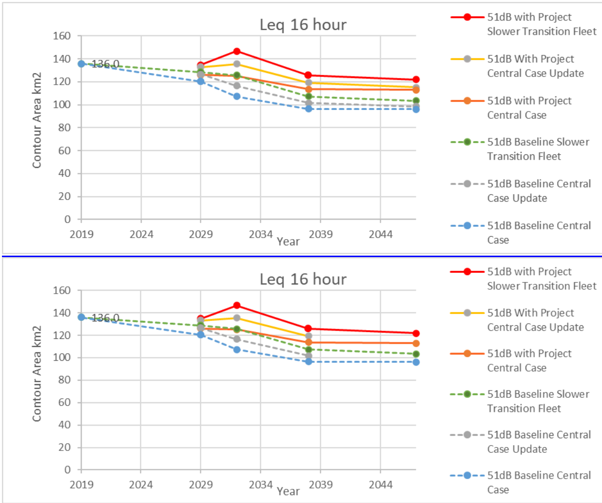
Diagram 3.1: Leq, 16 hour Day Contour Areas: 2019, 2029, 2032, 2038 and 2047
