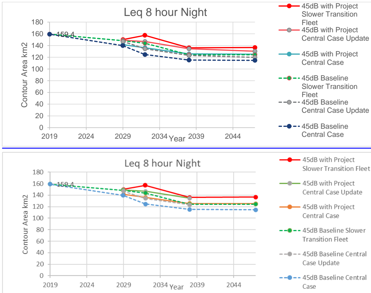
Diagram 3.2: Leq 8 hour Night Contour Areas: 2019, 2029, 2032, 2038 and 2047
